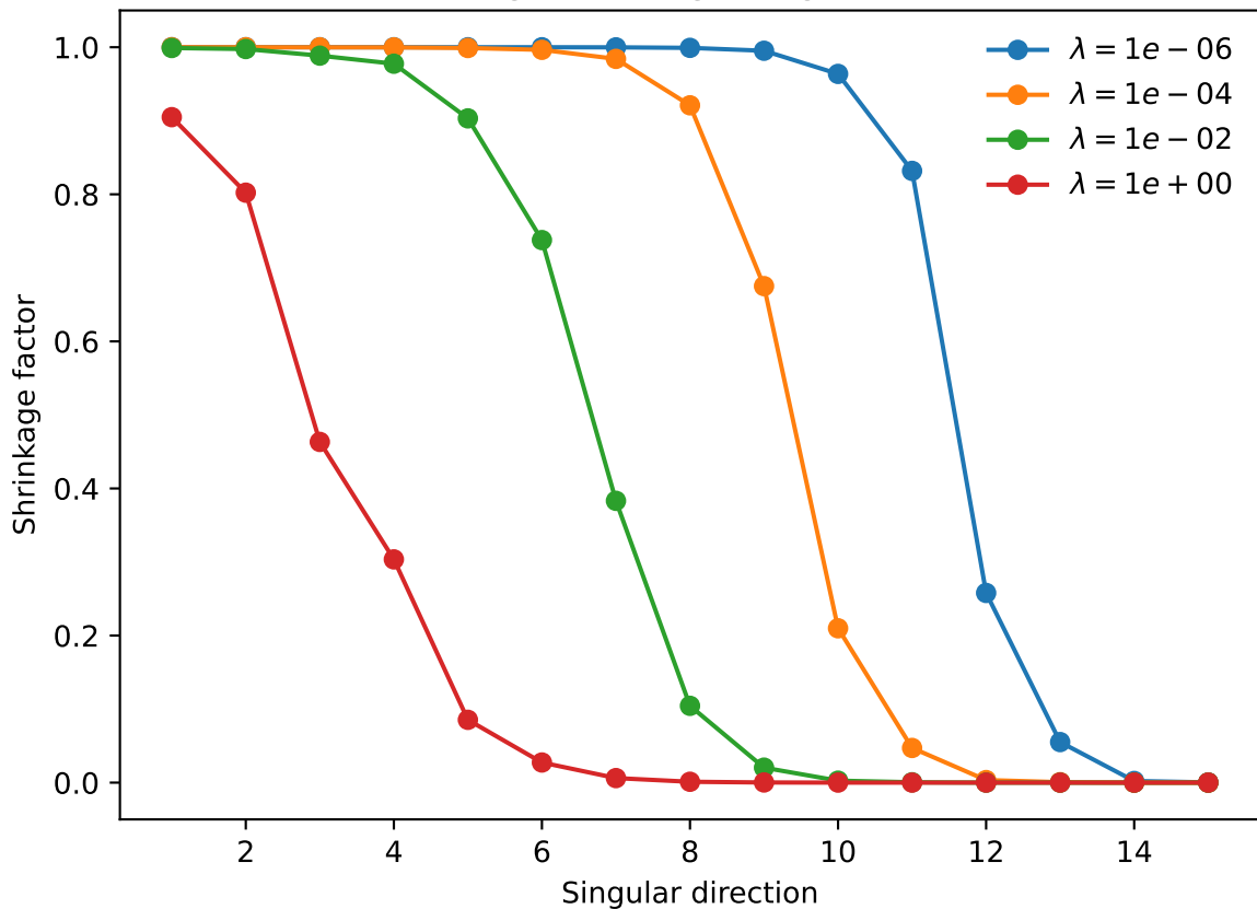
Ridge shrinkage, degree 15
