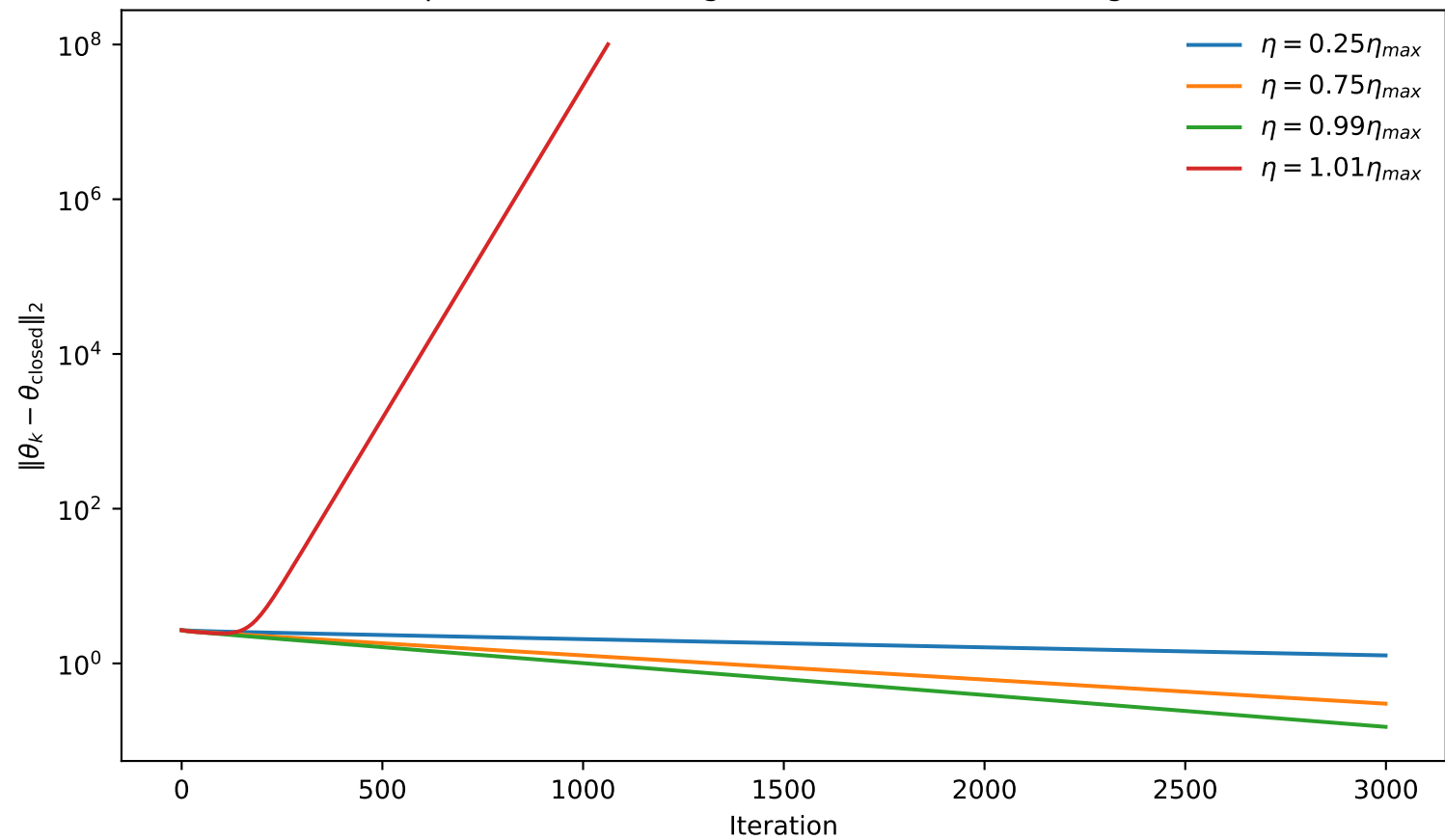
OLS parameter convergence for different learning rates
