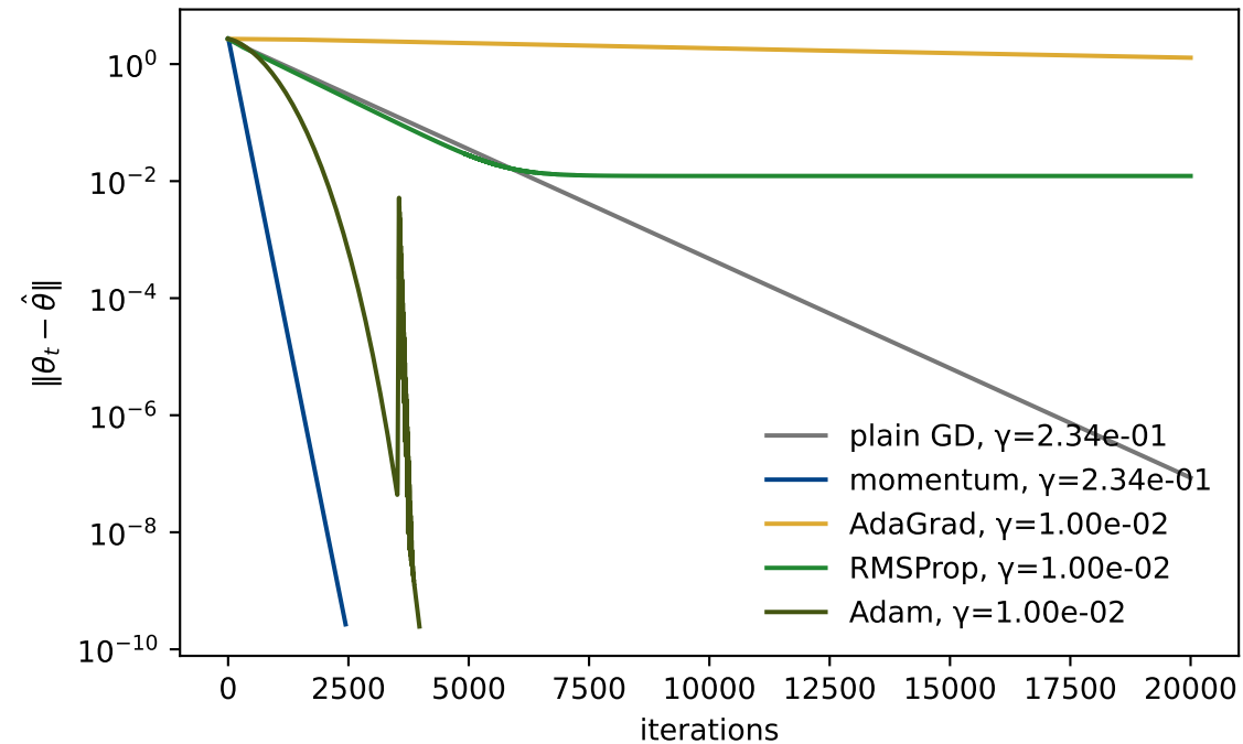
OLS
