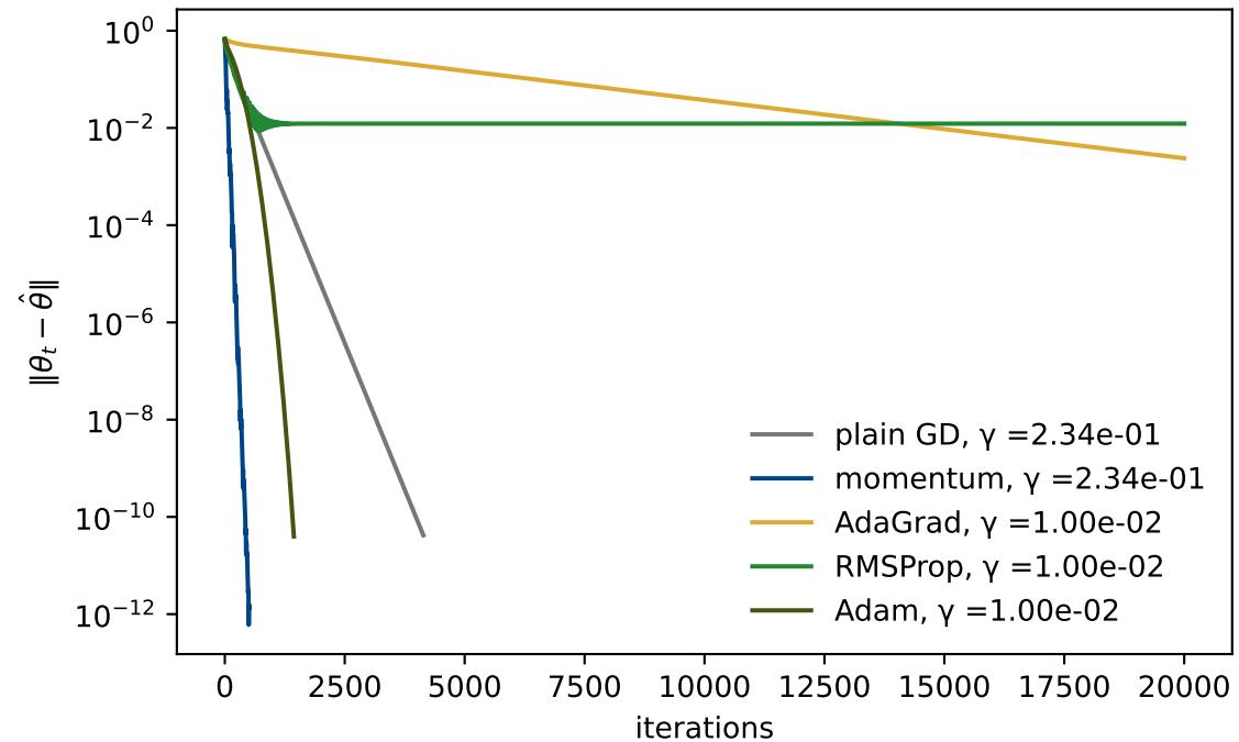
Ridge
