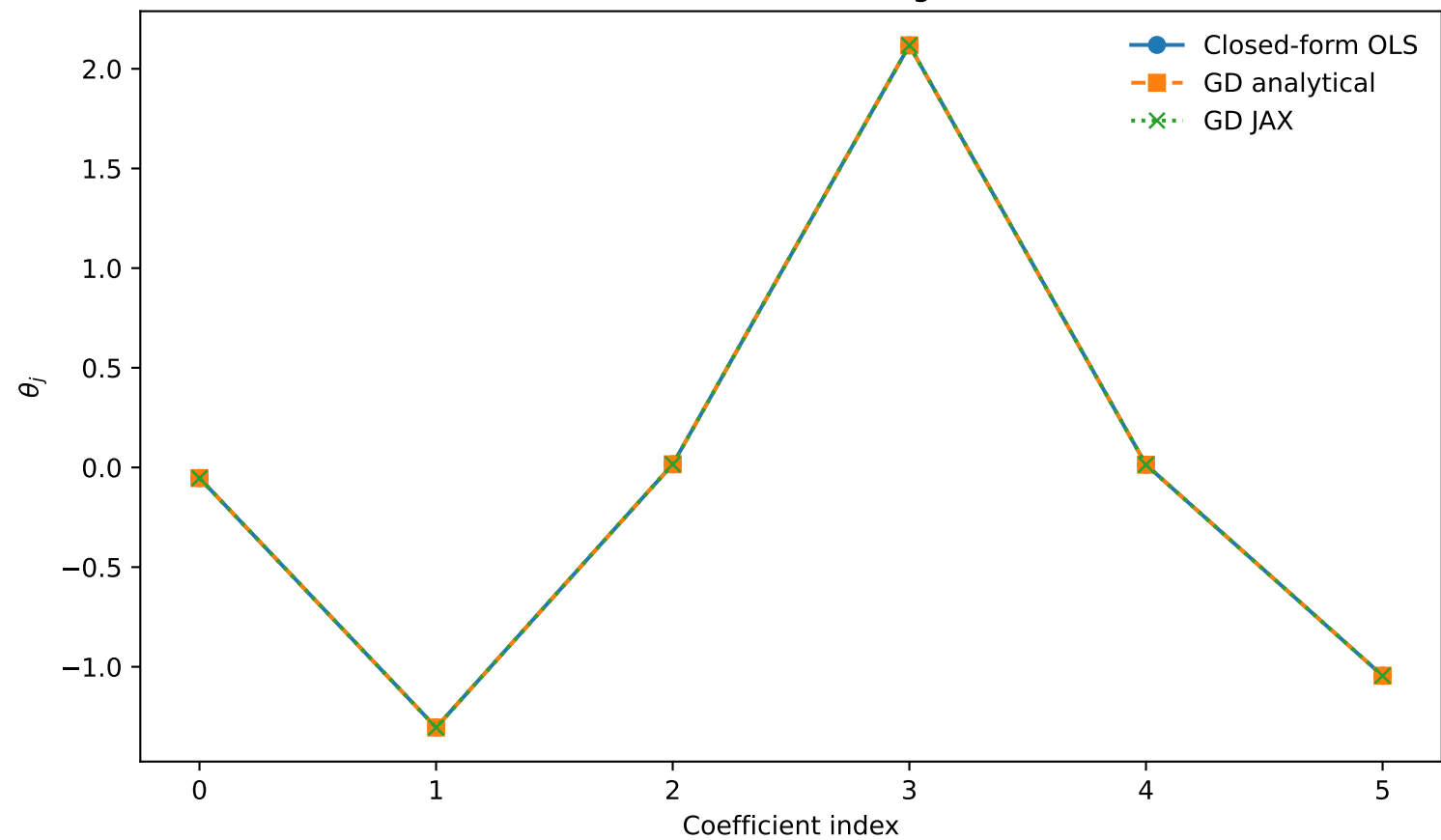
OLS coefficients: closed form vs gradient descent
