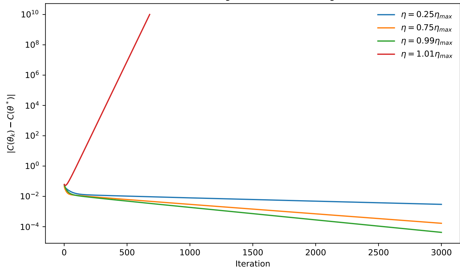
Effect of learning rate on OLS convergence
