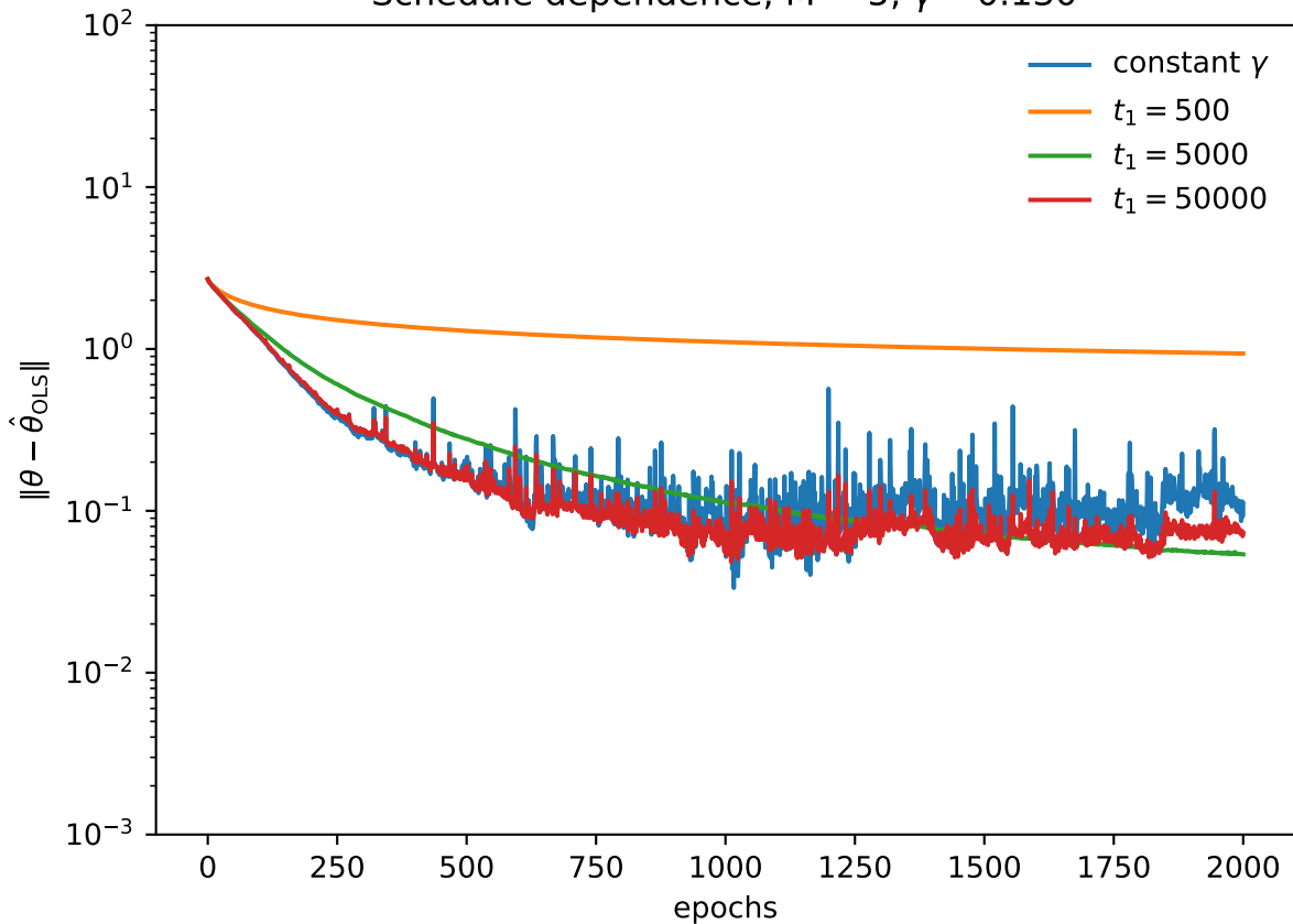
Schedule dependence, M = 5 , \gamma = 0.130
