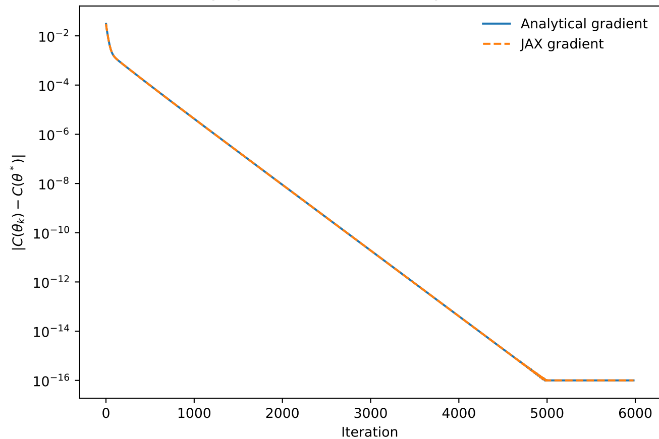
Ridge gradient descent convergence, \lambda = 0.01
