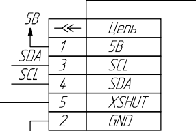
A10 Raspberry Pi 5
