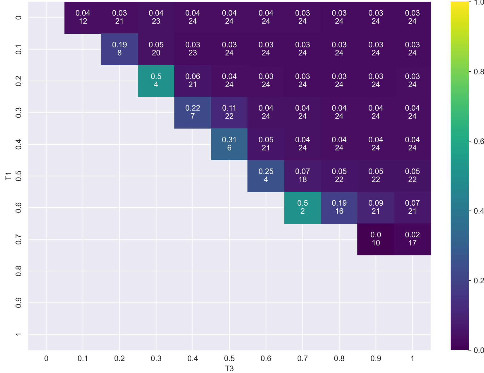
Macro Precision: Heatmap
