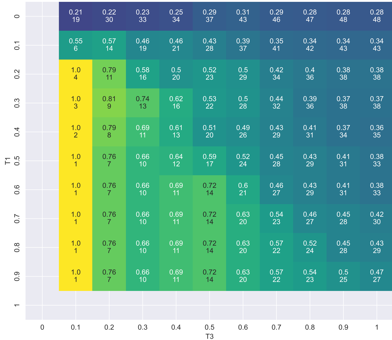
Macro Precision: Heatmap
