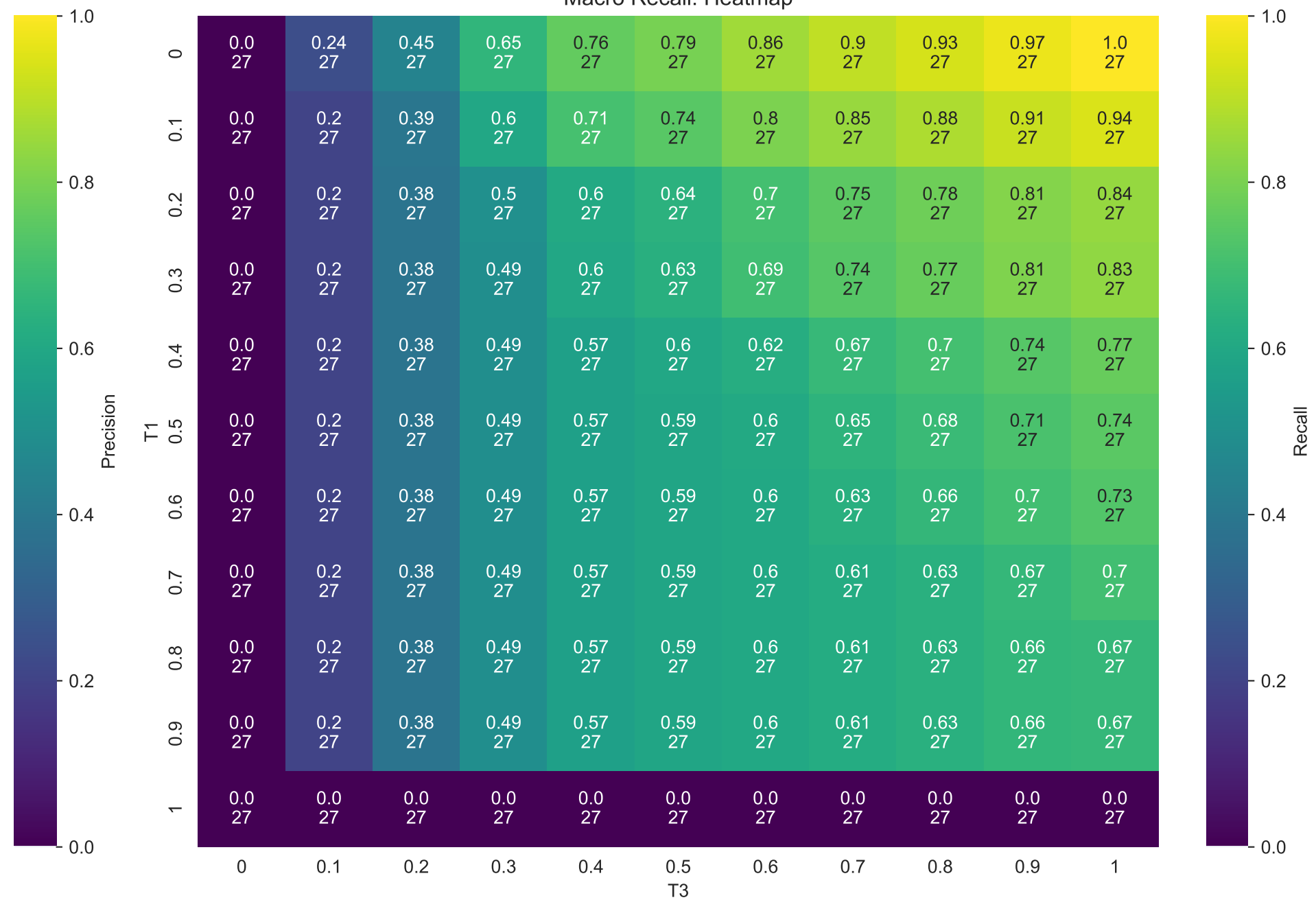
Macro Recall: Heatmap
