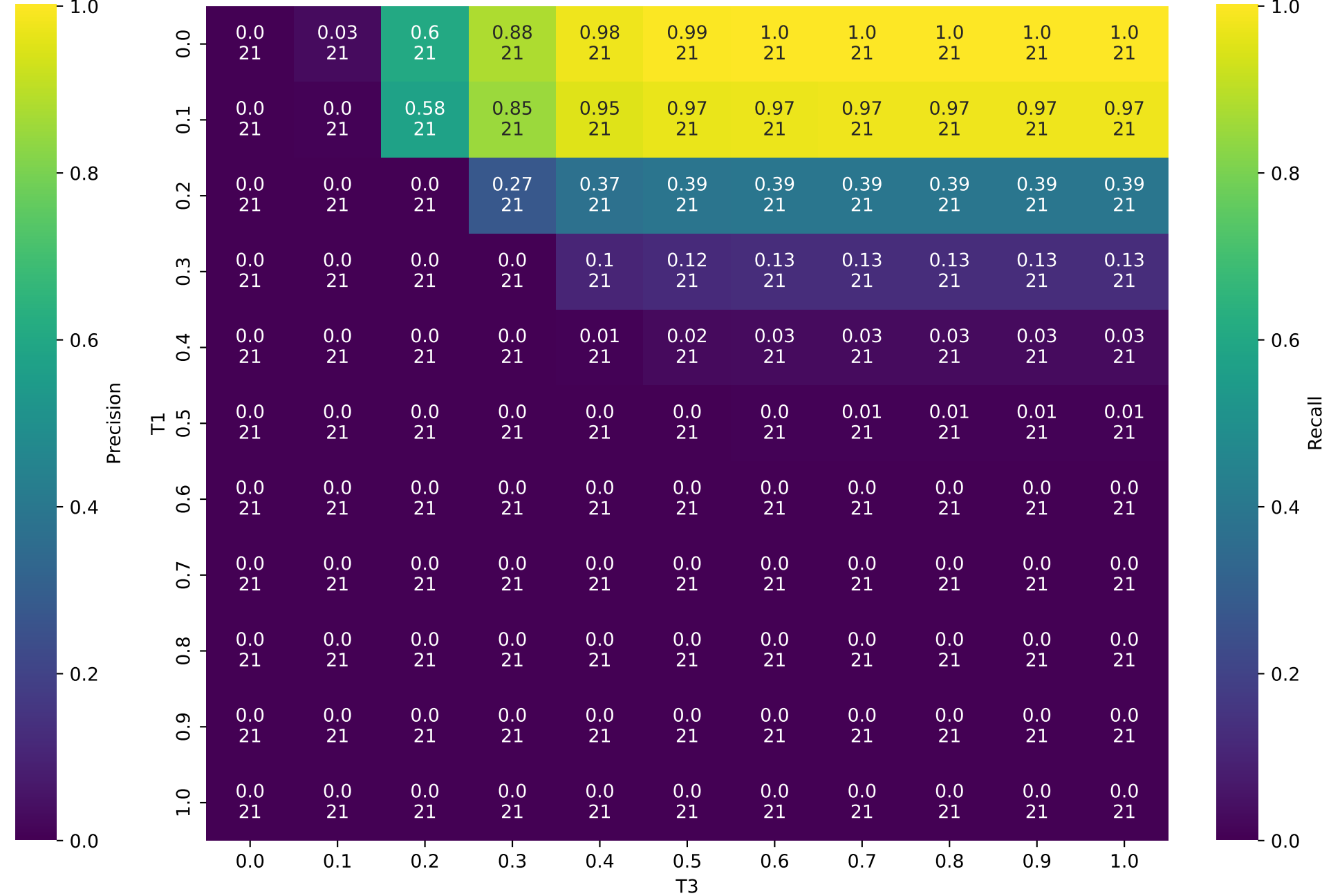
Macro Recall: Heatmap
