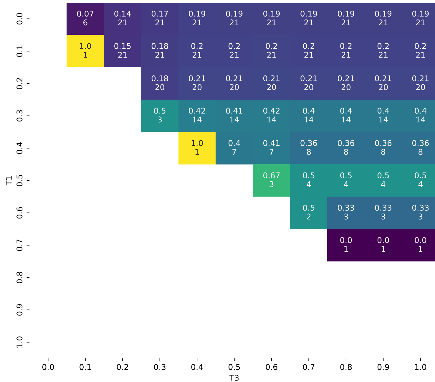
Macro Precision: Heatmap
