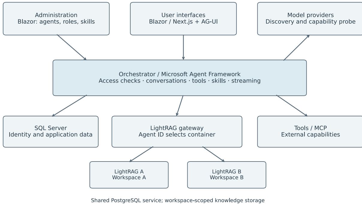
Figure 1: System overview derived from the inspected implementation. Dedicated LightRAG containers use agent-specific workspaces within shared PostgreSQL infrastructure.
