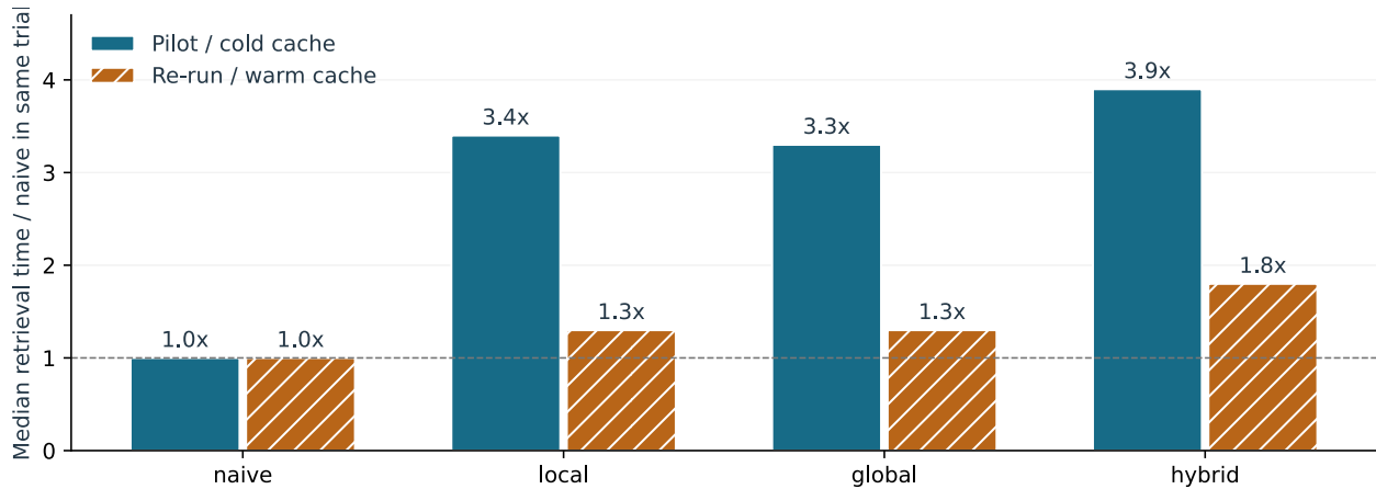
Figure 6: Reported relative median retrieval latency. Each trial has its own naive = 1 baseline; bar differences across trials are not absolute time savings. Source: retrieval trials, pp. 4–7.
