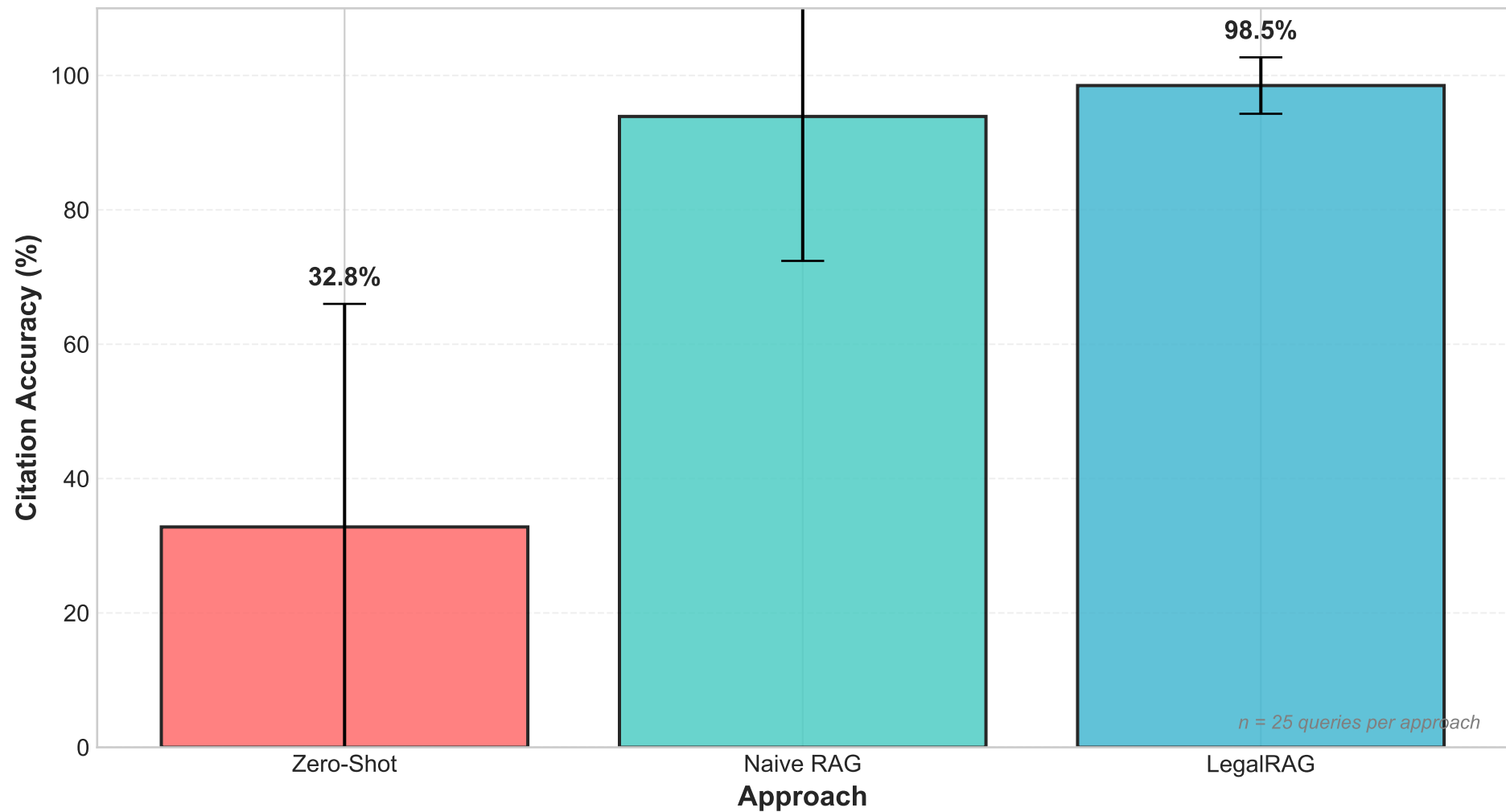
Citation Accuracy Across Approaches
