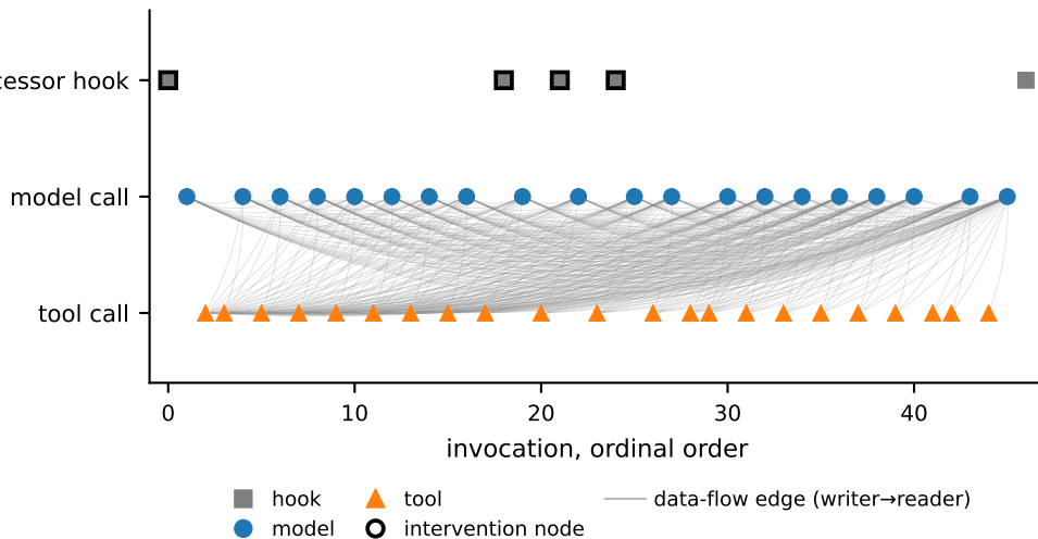
Rendered cone as injected, task 7619a514 (R1): 47 invocations, 409 edges, 15,566 bytes
