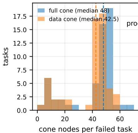
Cone size, 56 failed fresh tasks
