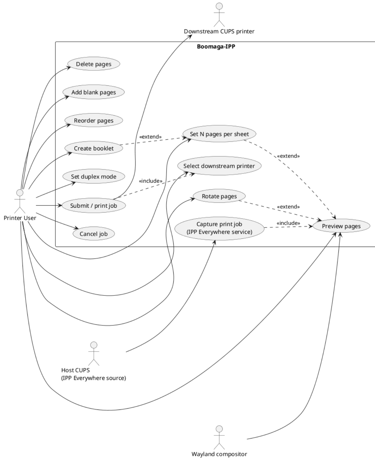
Boomaga-IPP — Use Case Diagram (conforms to code @ 34652fa)
