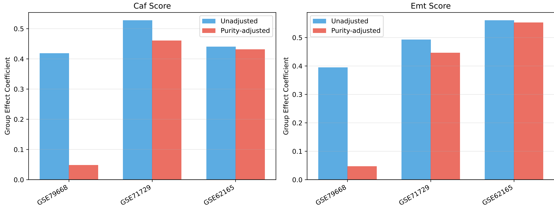
Purity-Adjusted CAF/EMT Effects (Figure 3E)
