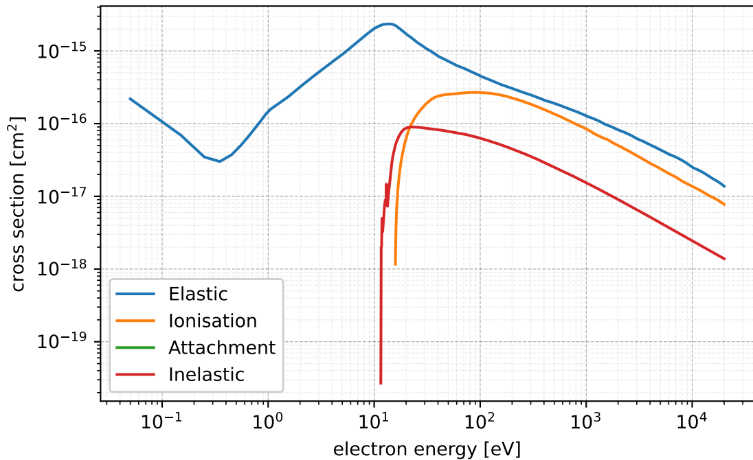
Argon Cross Section
