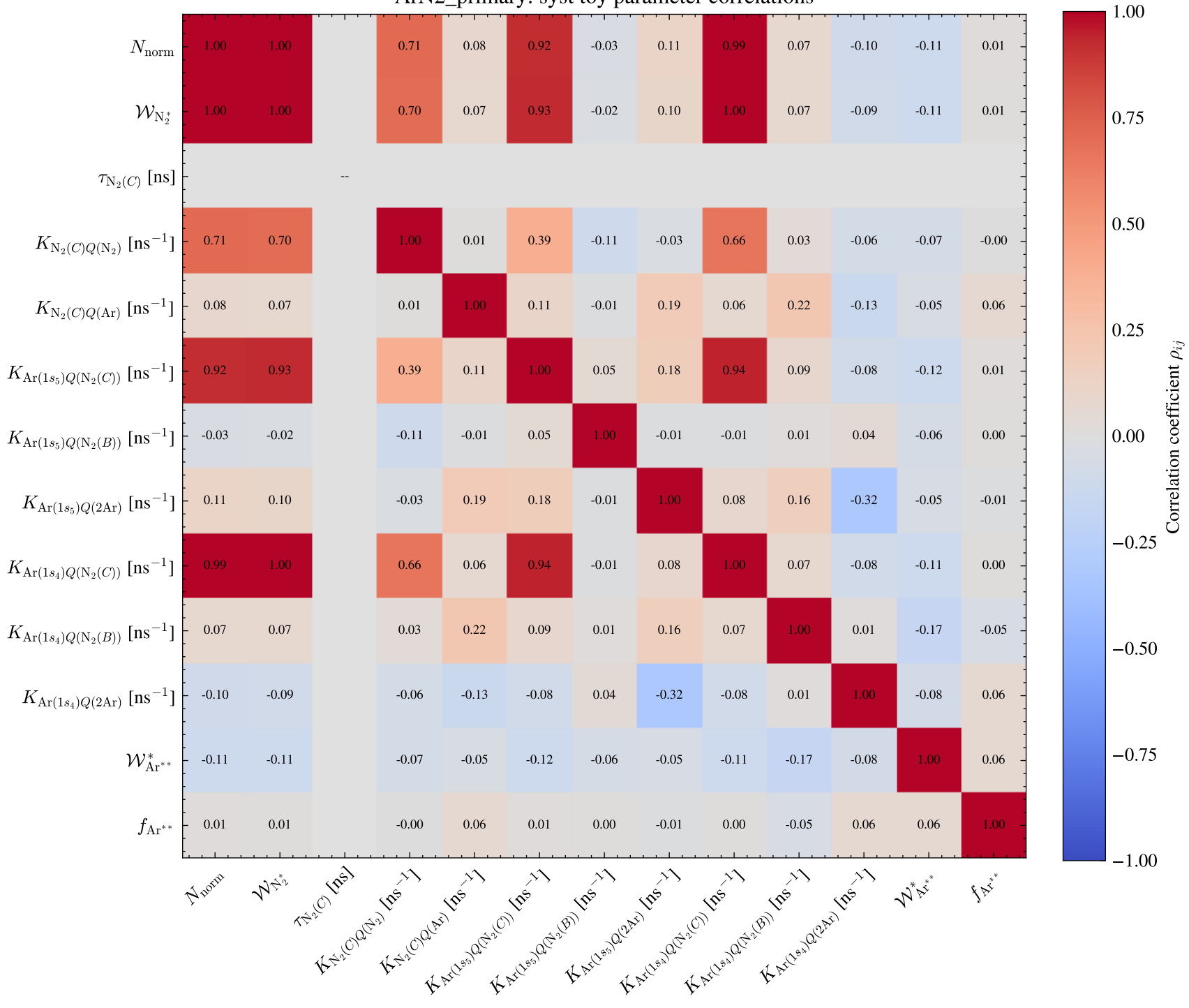
ArN2_primary: syst toy parameter correlations
