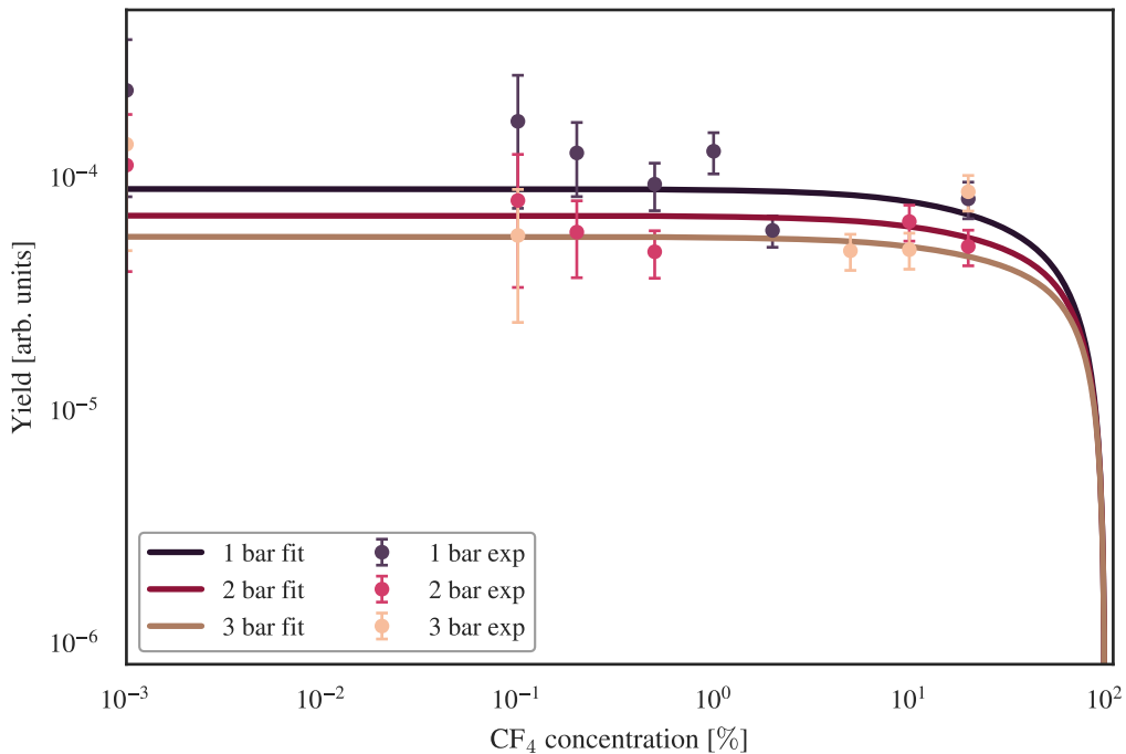
Ar-CF 4 primary IR fit, 727 nm
