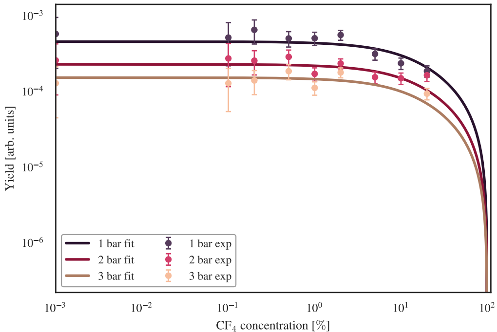
Ar--CF 4 primary IR fit, 750 nm
