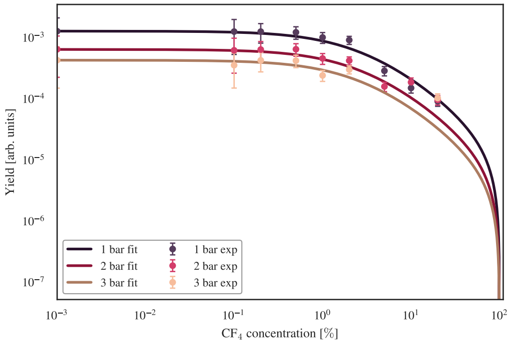
Ar-CF 4 primary IR fit, 763 nm
