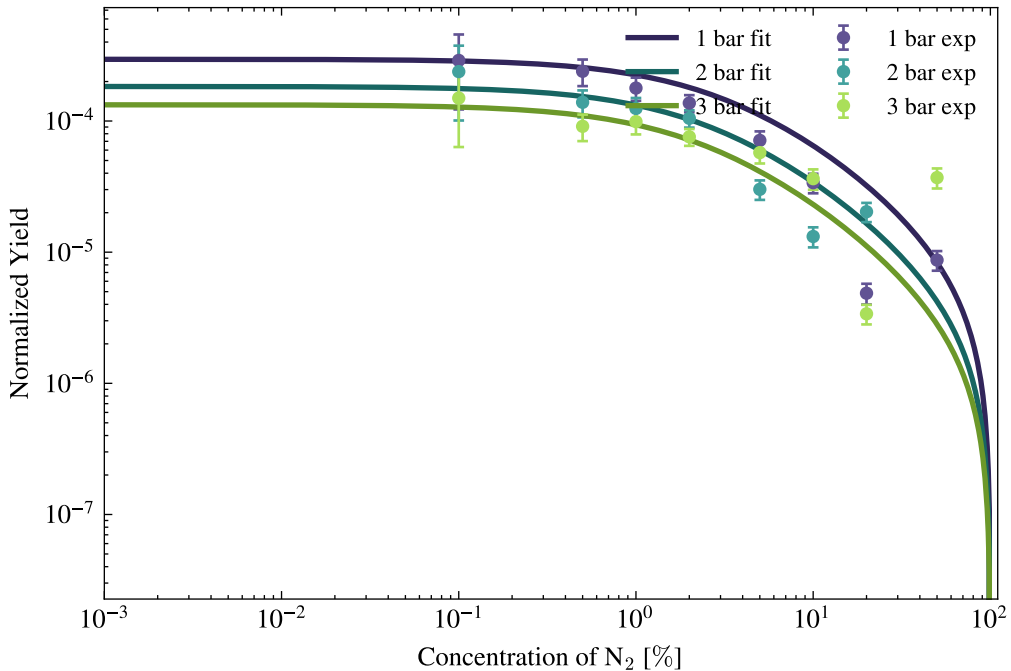
Primary ArN 2 IR (727 nm) Yield fit
