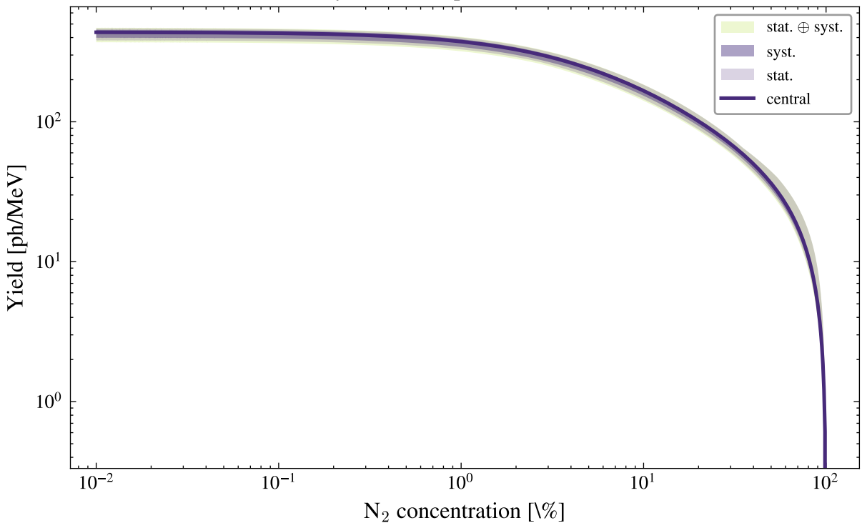
Primary Ar--N 2 IR prediction, 1000 mbar
