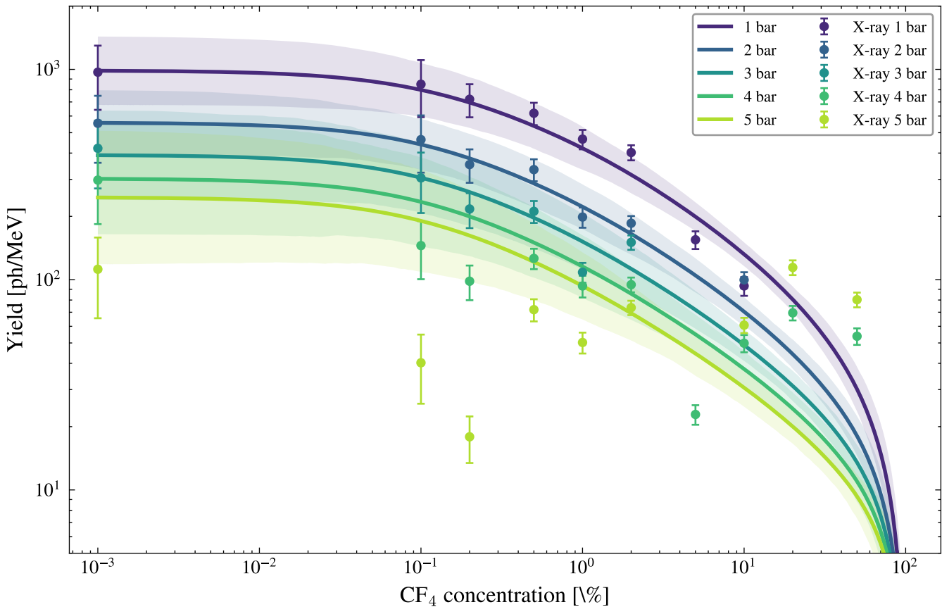
Primary Ar--CF 4 IR prediction, 1--5 bar
