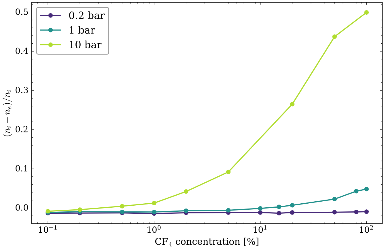
Ar--CF 4 GEM charge balance
