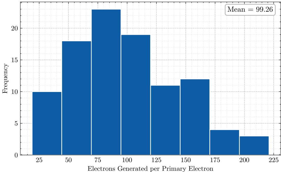
Electron Gain ar 95.0% - cf4 5.0% 0.2 bar 44.5 kV/cm
