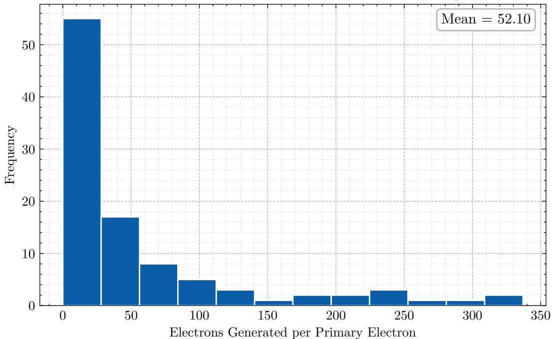
Electron Gain ar 99.0% - cf4 1.0% 10.0 bar 97.9 kV/cm
