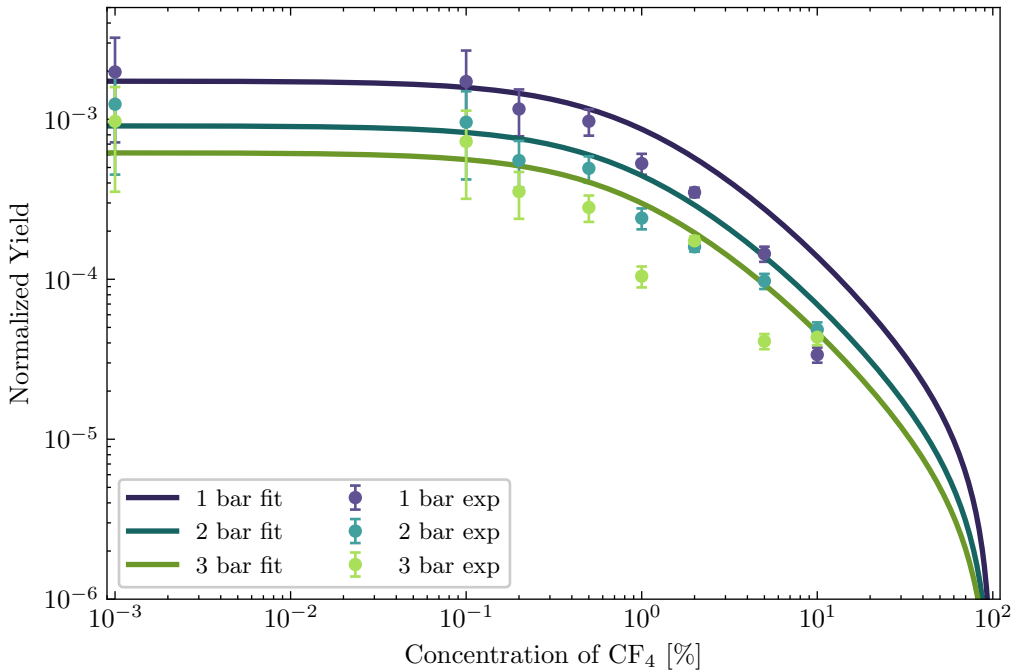
Primary ArCF 4 IR (772 nm) Yield fit
