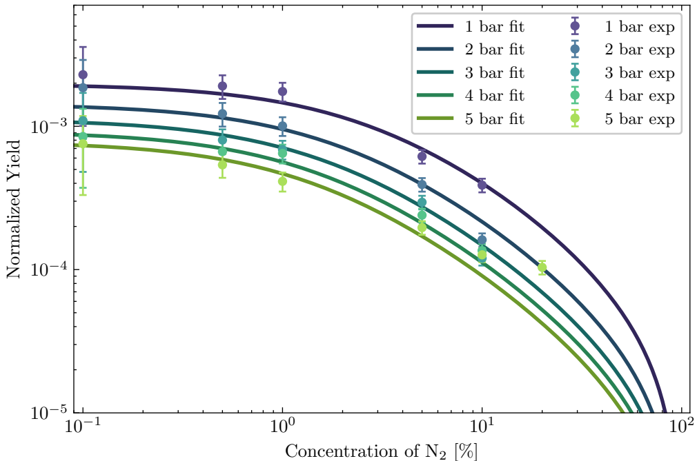
Primary ArN 2 IR (772 nm) Yield fit
