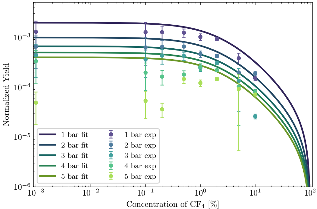
Primary ArCF 4 IR (763 nm) Yield fit
