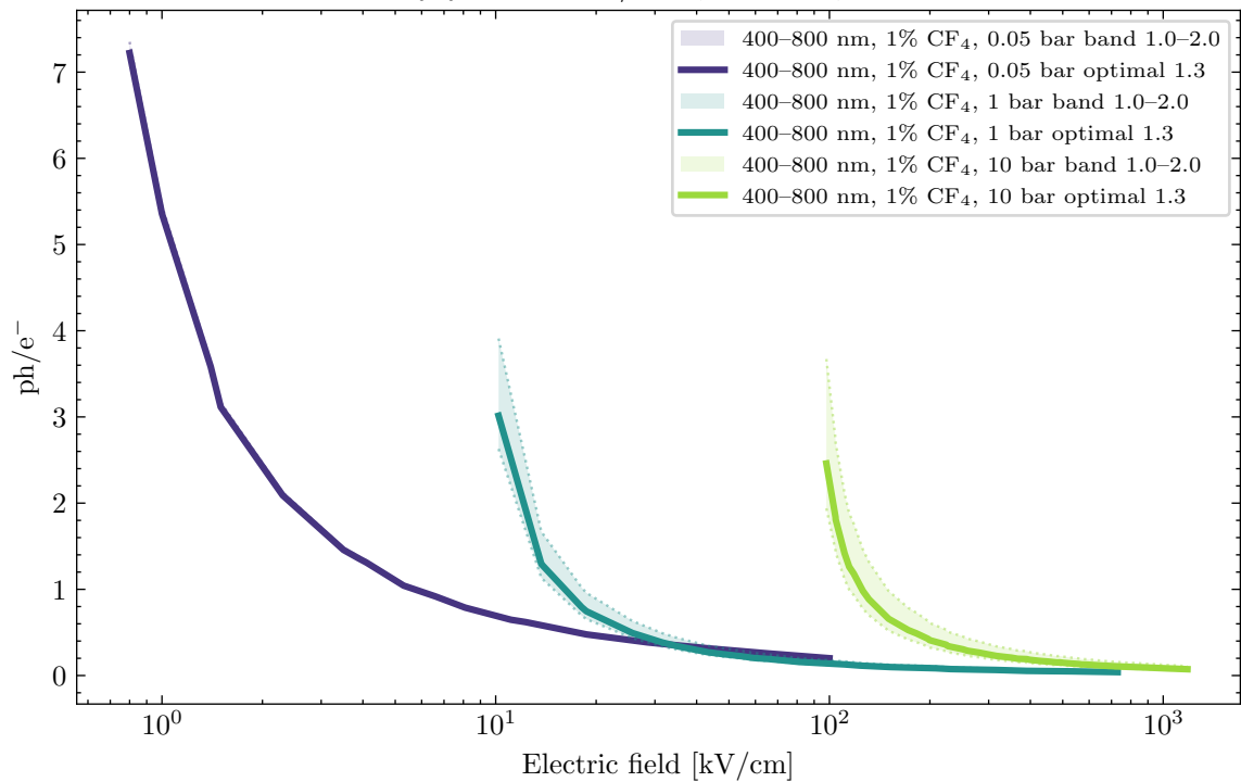
Secondary yield for Ar/CF 4 , 1% CF 4 , 400–800 nm
