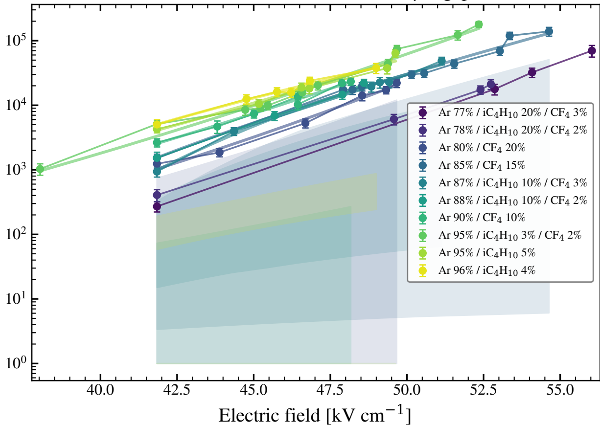
Gain vs electric field (1 bar, 150 \mu\text{m} gap)
