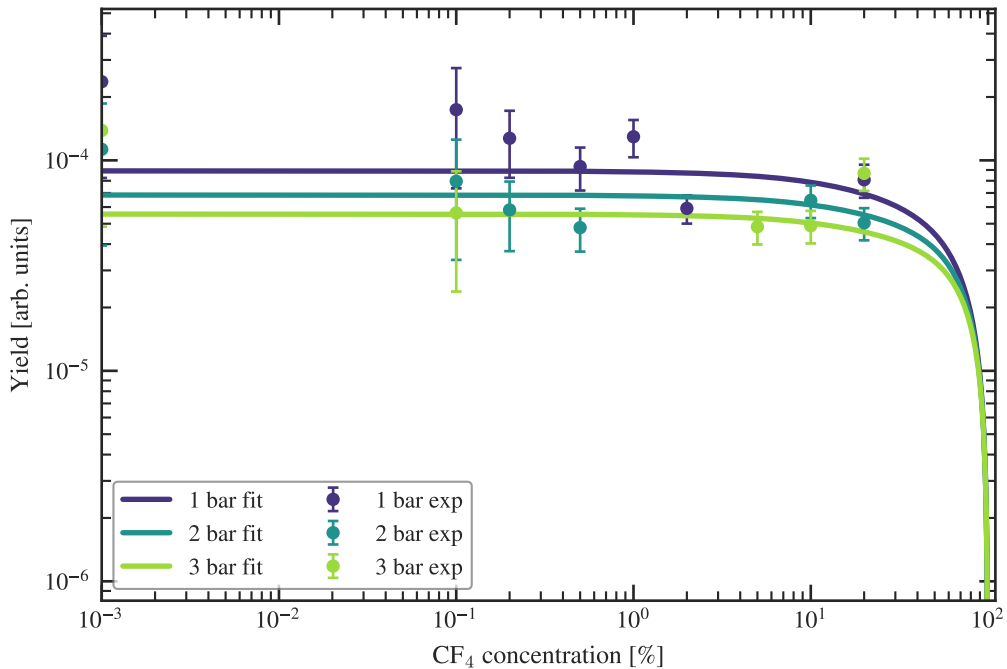
Ar--CF 4 primary IR fit, 727 nm
