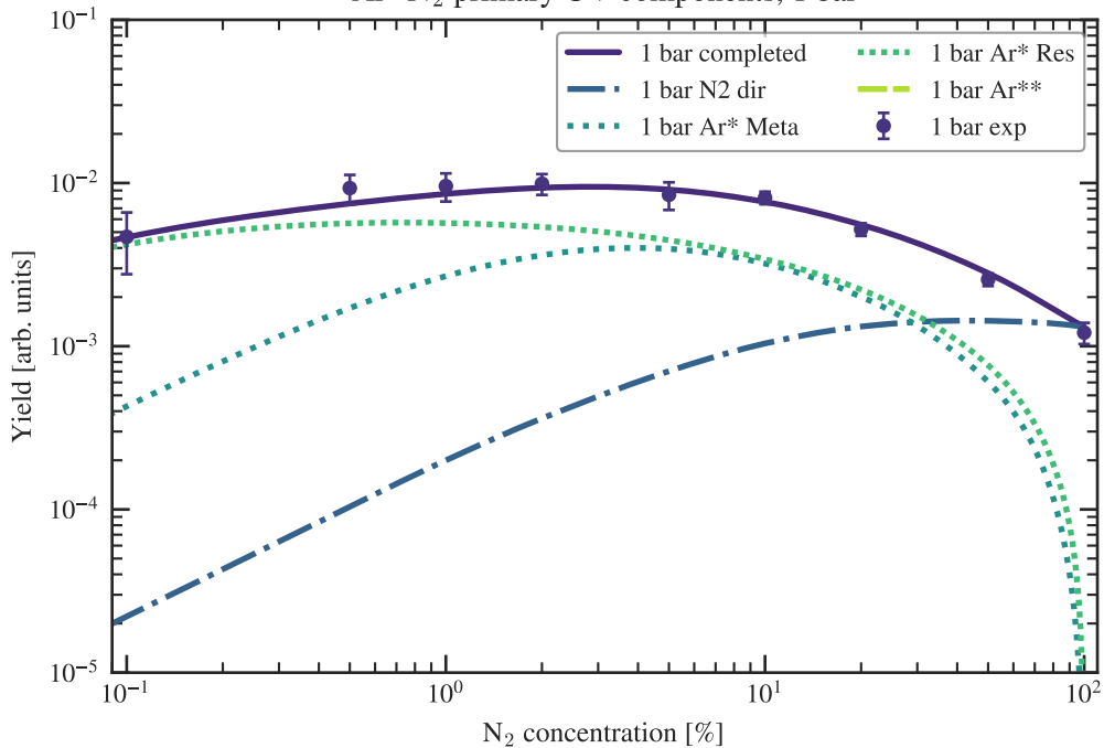
Ar--N 2 primary UV components, 1 bar
