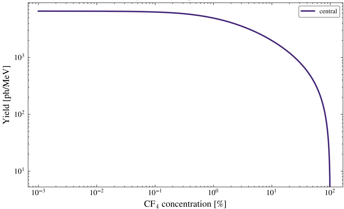
Primary Ar--CF 4 IR prediction, 50 mbar
