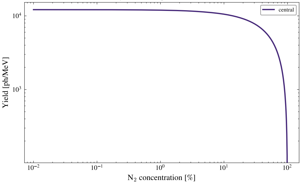
Primary Ar--N 2 IR prediction, 0.1 mbar
