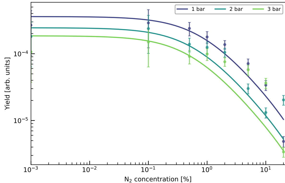
Joint IR fit: ArN 2 , 727 nm
