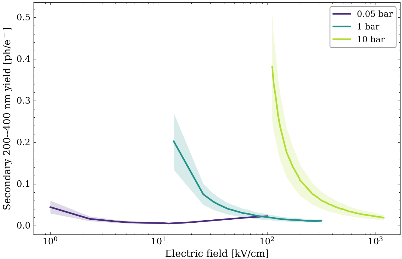
Secondary Ar--CF 4 UV (200--400 nm) vs E, 1% CF 4 , N_e = 100 \pm 20
