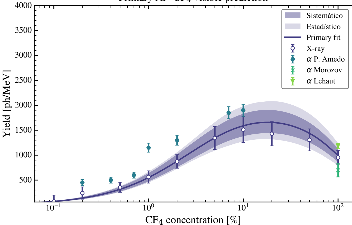
Primary Ar--CF 4 visible prediction
