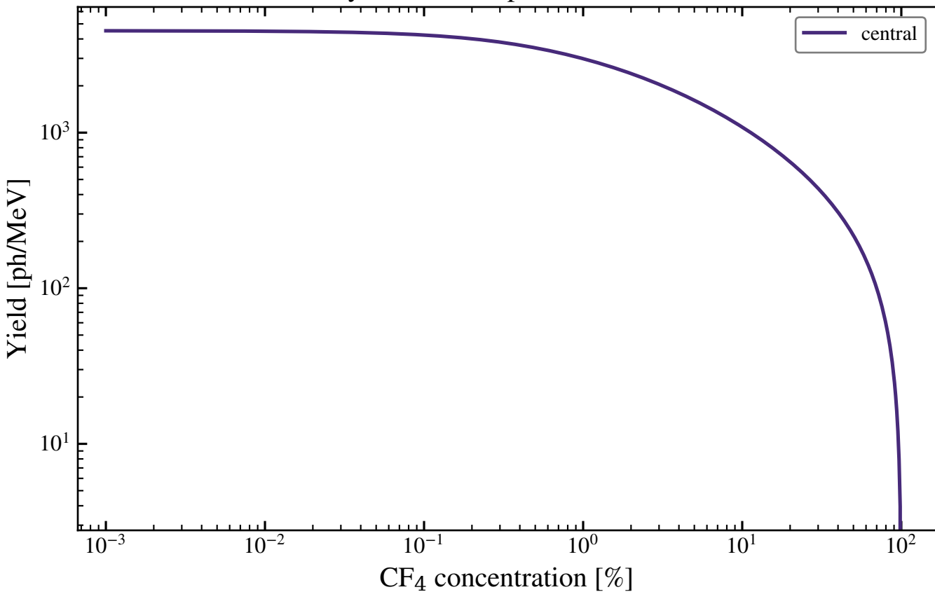
Primary Ar--CF 4 IR prediction, 100 mbar
