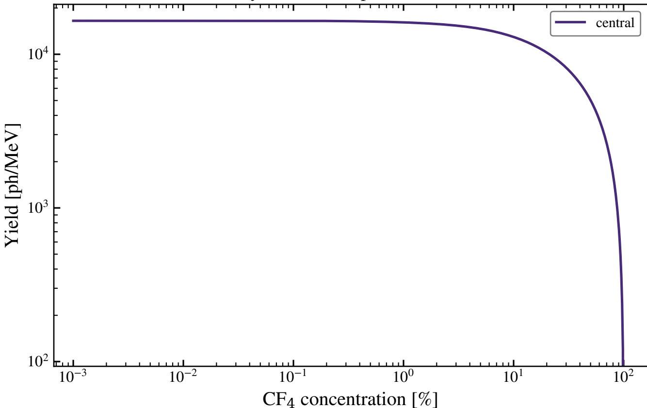
Primary Ar--CF 4 IR prediction, 1 mbar
