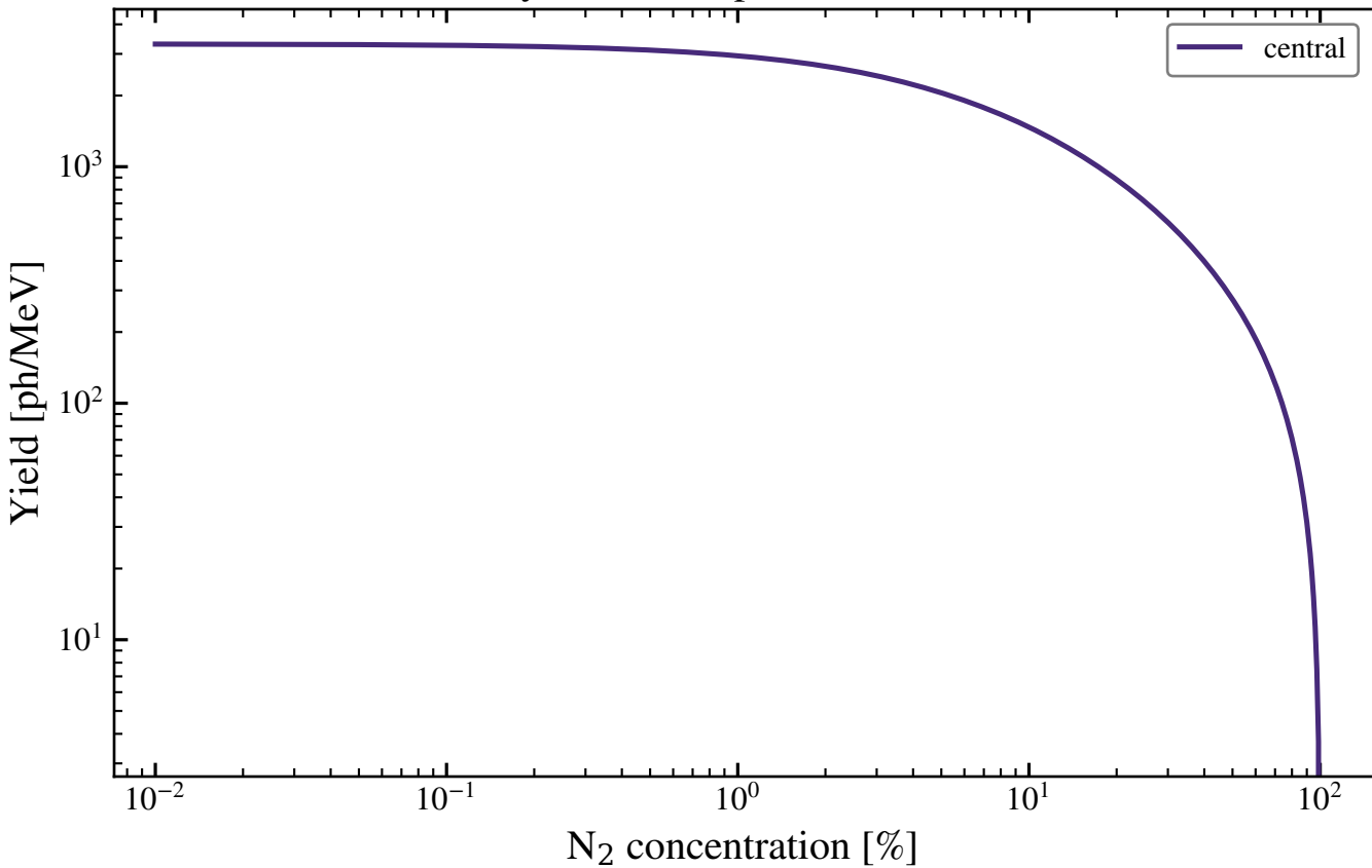
Primary Ar--N 2 IR prediction, 100 mbar
