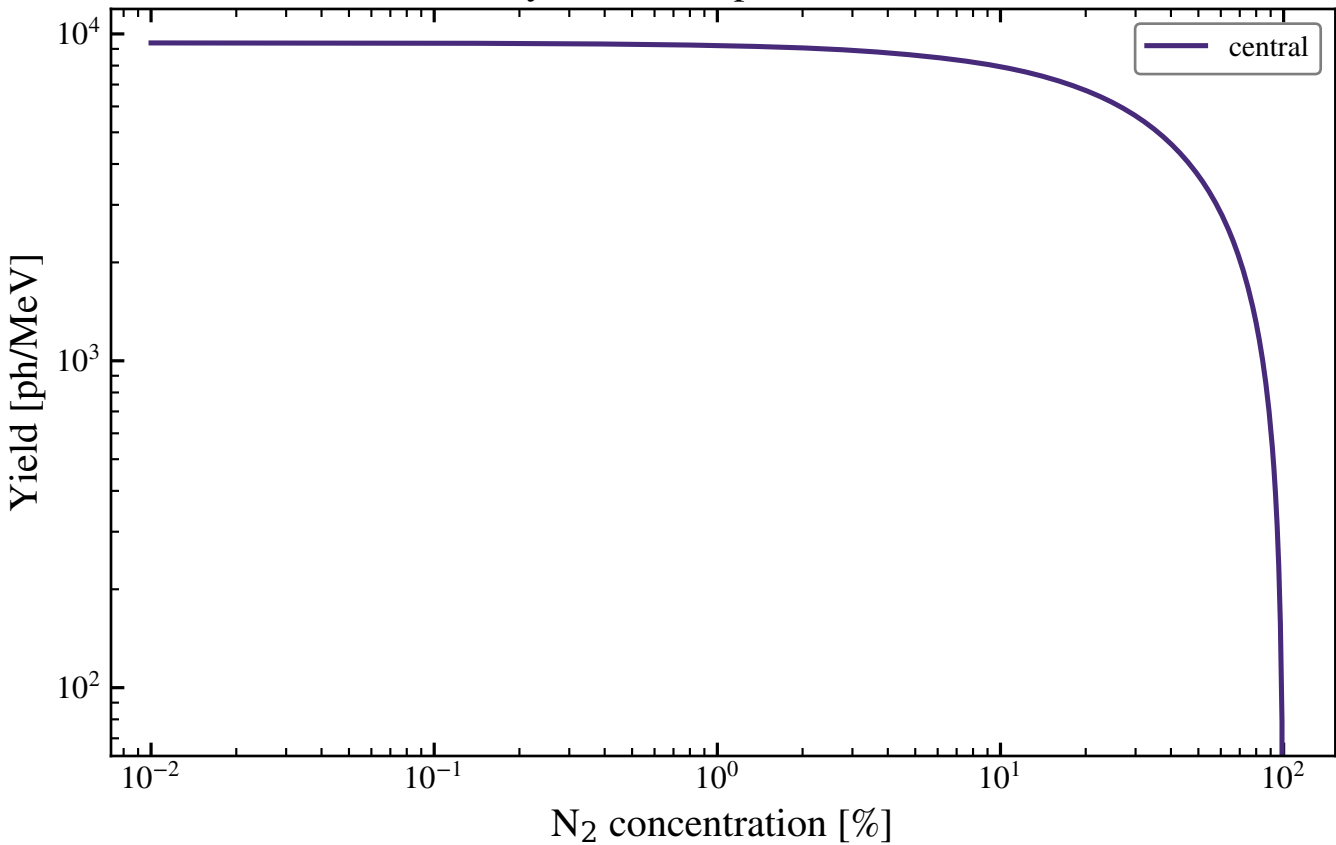
Primary Ar--N 2 IR prediction, 1 mbar
