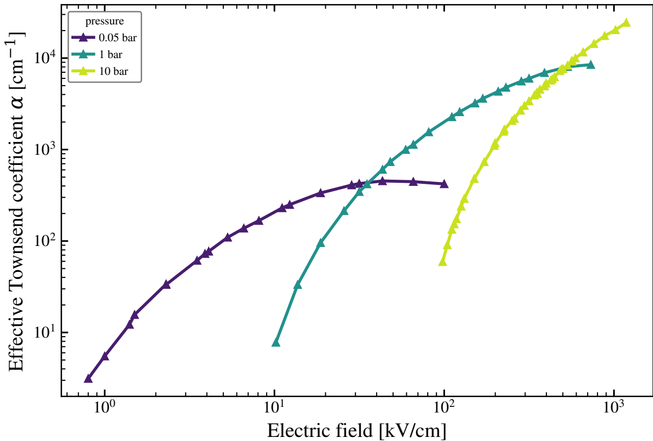
Ar 99 / CF 4 1%: \alpha vs E
