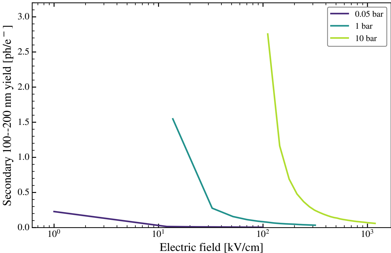
Secondary Ar--CF 4 VUV (100--200 nm) vs E, 1% CF 4 , N_e = 100 \pm 20
