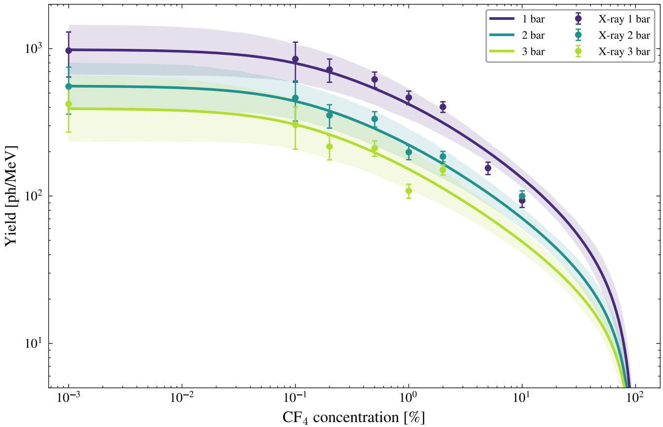
Primary Ar--CF 4 IR prediction, 1--3 bar
