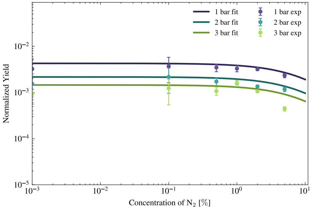
Primary ArN 2 IR (750 nm) Yield fit
