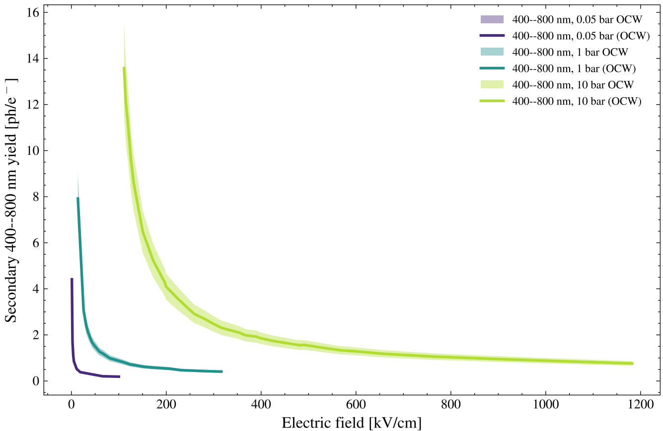
Secondary Ar--CF 4 400--800 nm vs E, 1% CF 4 , N_e = 100 \pm 20
