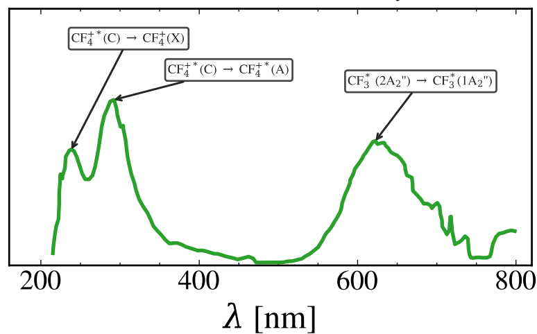
He--CF 4 80/20 Secondary
