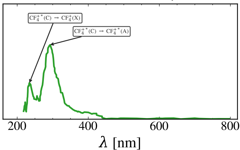
He--CF 4 80/20 Primary
