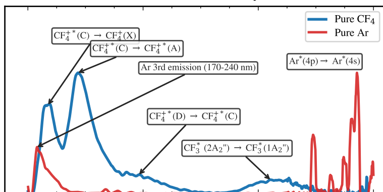
Pure CF 4 Primary
