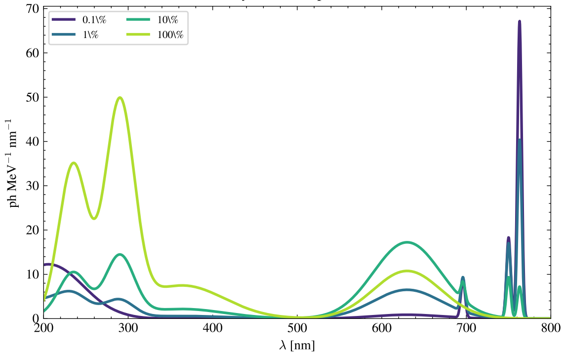
Primary Ar--CF 4 spectra, 1 bar
